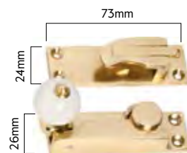
I604 PB
