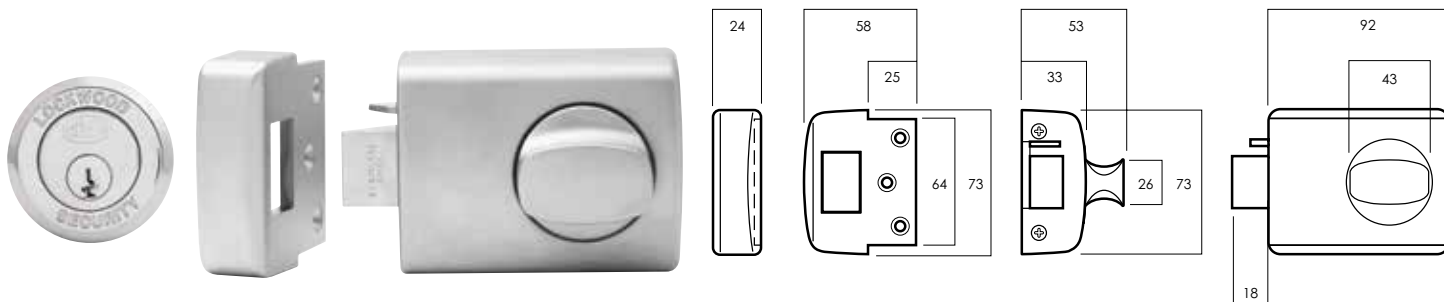
Exterior Cylinder
