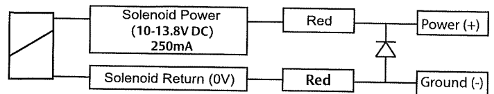
Fig. 3 - Electrical Schematic
